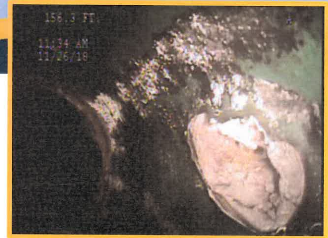
Cucamonga Trunk Sewer Structural Damage
